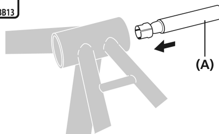
(A) TL-BB13
