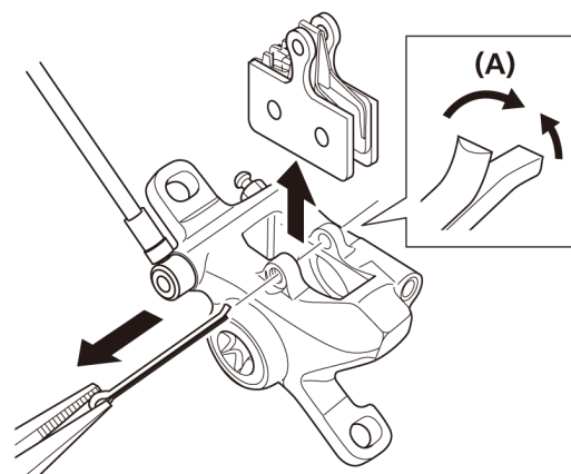
(A) Copiglia
