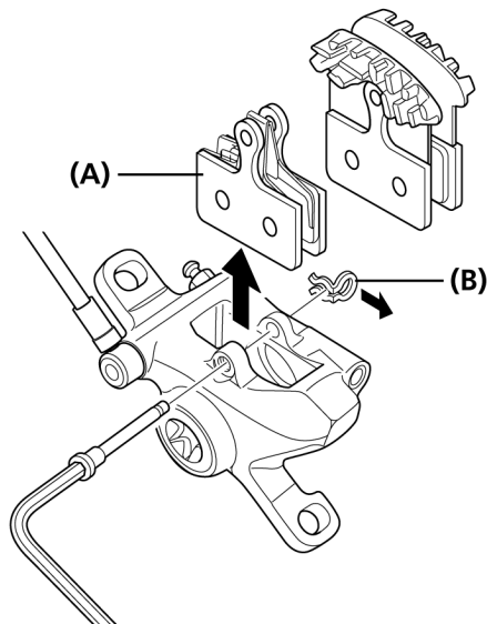
(A) Pastiglia freno (B) Anello a scatto
