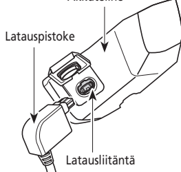
<BT-E6010> Akkuteline
