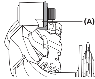
(A) Garra de tope
