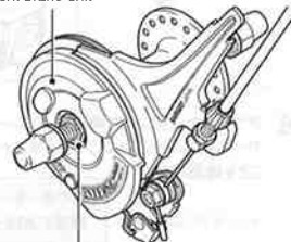
Brake unit fixing nut
