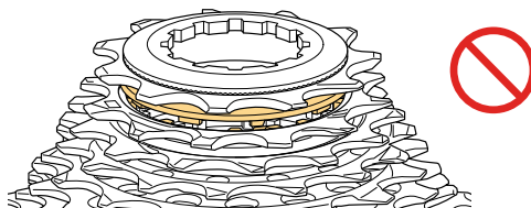
There are places where the protrusions on the smallest sprocket overlap the indents in the second sprocket.
