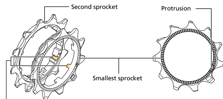
Align the protrusion with the groove.
