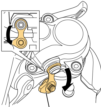
Plate unit rubber cap
