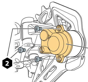
Plate unit cover
