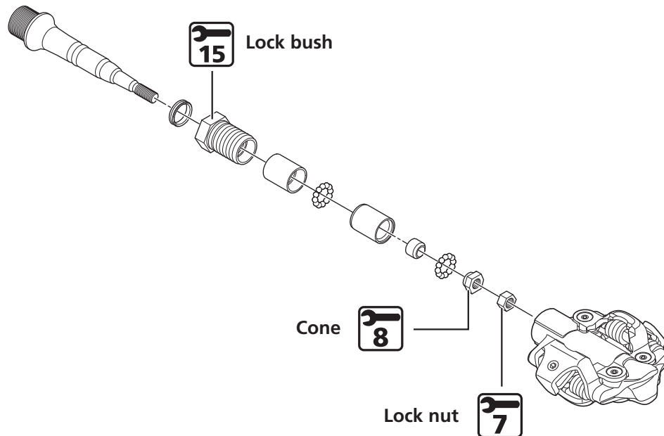
PD-M9100/PD-M9120
