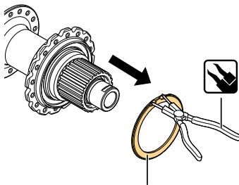
Snap ring with outer dust cover
