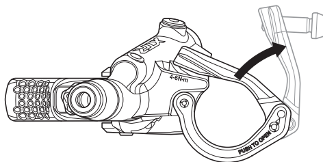
Brake lever with open clamp band
