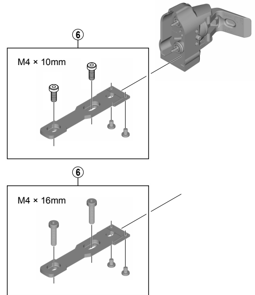
External / Internal type: Short size battery mount
