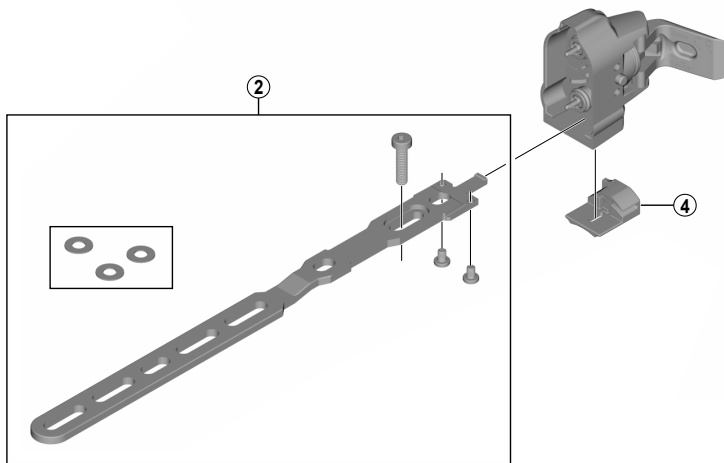
External type: Long size battery mount
