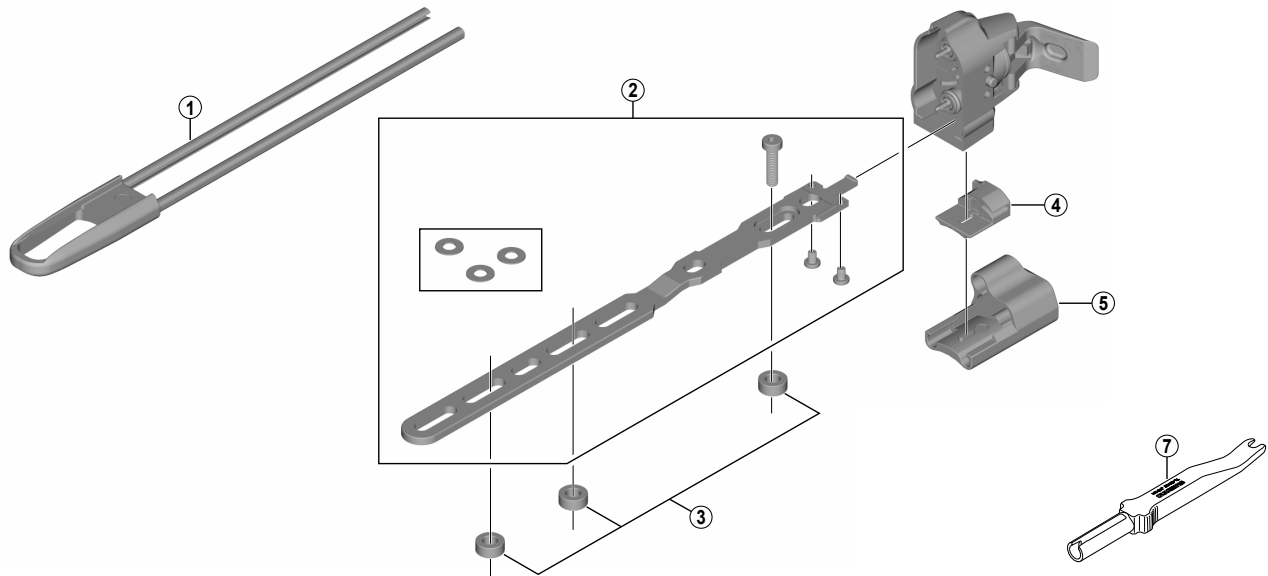
Internal type: Long size battery mount
